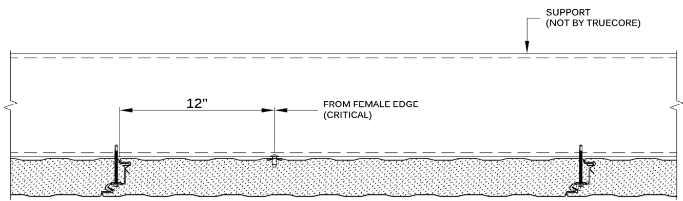
(FP2) SIDE JOINT AND (1) BULB-TITE® RIVET
