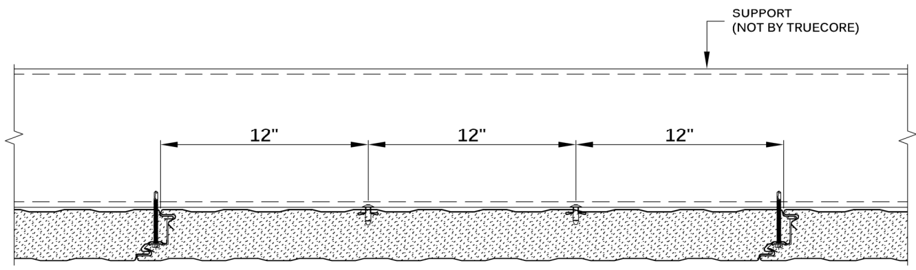
(FP3) SIDE JOINT AND (2) BULB-TITE® RIVETS
